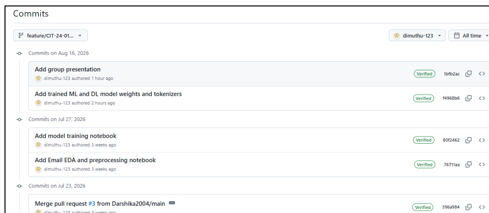
Figure 7: member 2 commits
