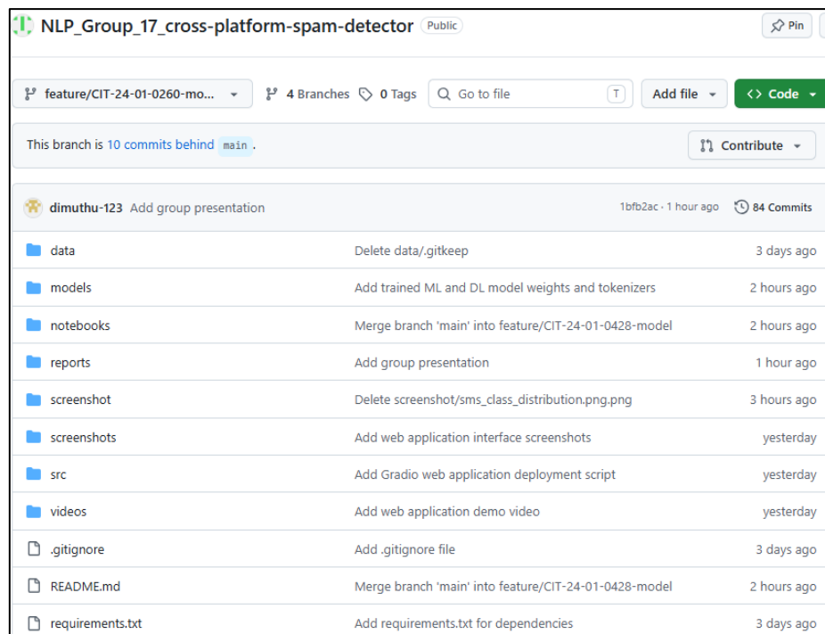
Figure 6:member 2 branch
