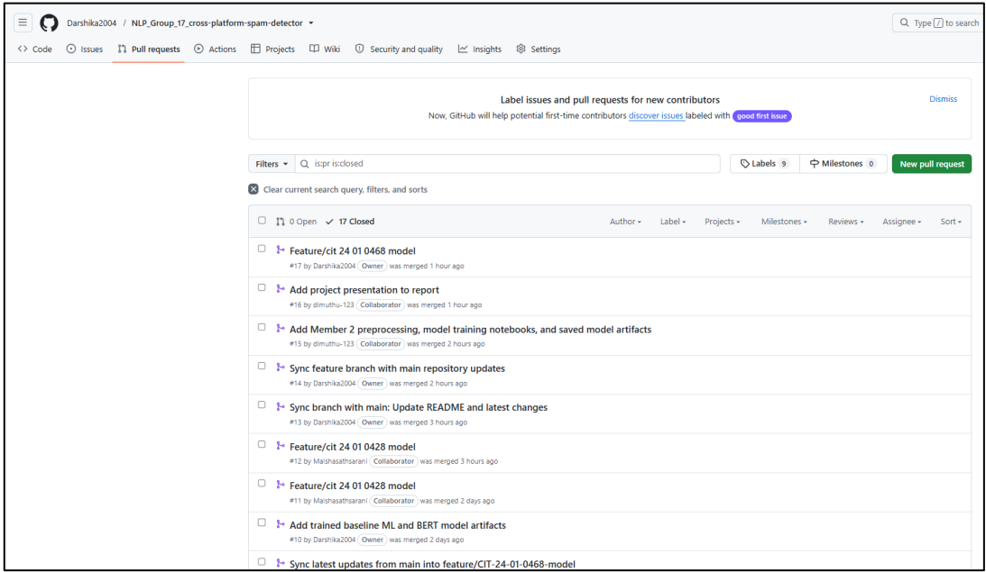
Figure 10: Merge Evidence
