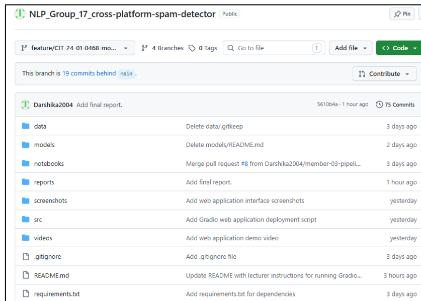
Figure 8: member 3 branch
