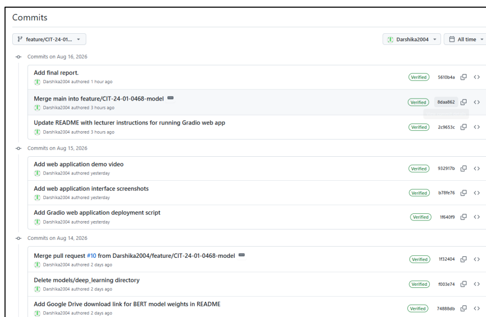
Figure 9:member 3 commits
